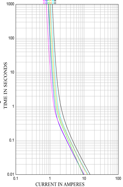
Average Time Current (I-T Curves)
